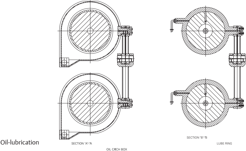
OIL CATCH BOX
