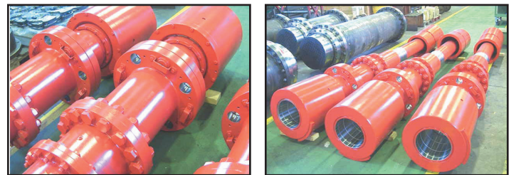
Spindles with shear pins
